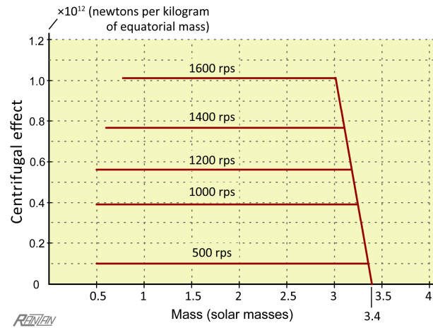
Figure 6. Centrifugal "force" is plotted as a function of the mass for several spin rates. The sloping line traces the centrifugal effect attenuation. Notice that if the mass corresponds to 3.4, then it will manifest no centrifugal effect whatsoever —regardless of spin rate. (Sphericity and constant radius of 10,000 meters is assumed.)
