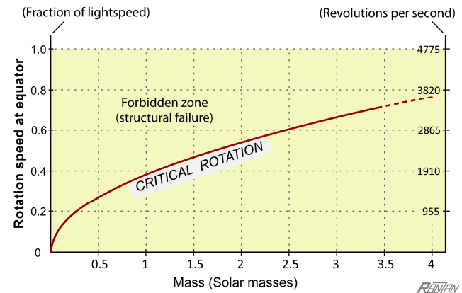
Figure 1. Centrifugal effect increases with rotation; but the rotation rate, in accordance with the conventional view, imposes a limit. The curve traces the critical combination of mass and spin for ten-kilometer-radius structures; combinations where the gravity and centrifugal effects are in balance. Above the curve, structures lose their gravitational cohesion.
