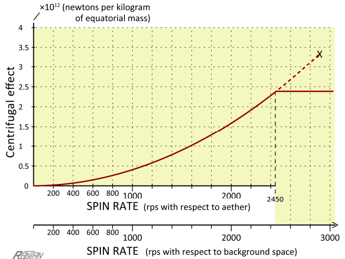
Figure 5. Centrifugal "force" is plotted as a function of the spin rate, thereby giving a graphic demonstration of the centrifugal effect attenuation principle . When the 2.5-solar-mass neutron star discussed in the text finds itself spinning at 2450 revolutions per second, the centrifugal effect reaches a limit — 2.37 \times 10^{12} newton for each kilogram of equatorial mass. This "force" limit remains constant regardless of any further increase in the spin rate. The dashed portion of the curve is an unrealistic extrapolation according to which special relativity is violated and the structure flies apart at 2900 rps indicated by the "X" mark.
