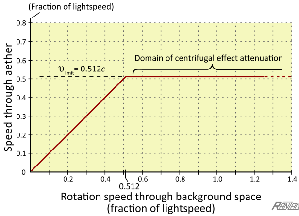
Figure 4. Graphic implications of conforming to the special relativity restriction. Two pieces of information are contained within this graph. First, it gives the limit of the equatorial speed through aether —as indicated by the horizontal line at 0.512 c . Second, the height of the curve gives the velocity magnitude for determining the centrifugal effect. (Again, the rotating structure to which these values apply is a 2.5-solar-mass neutron star of radius 10 kilometers.)
