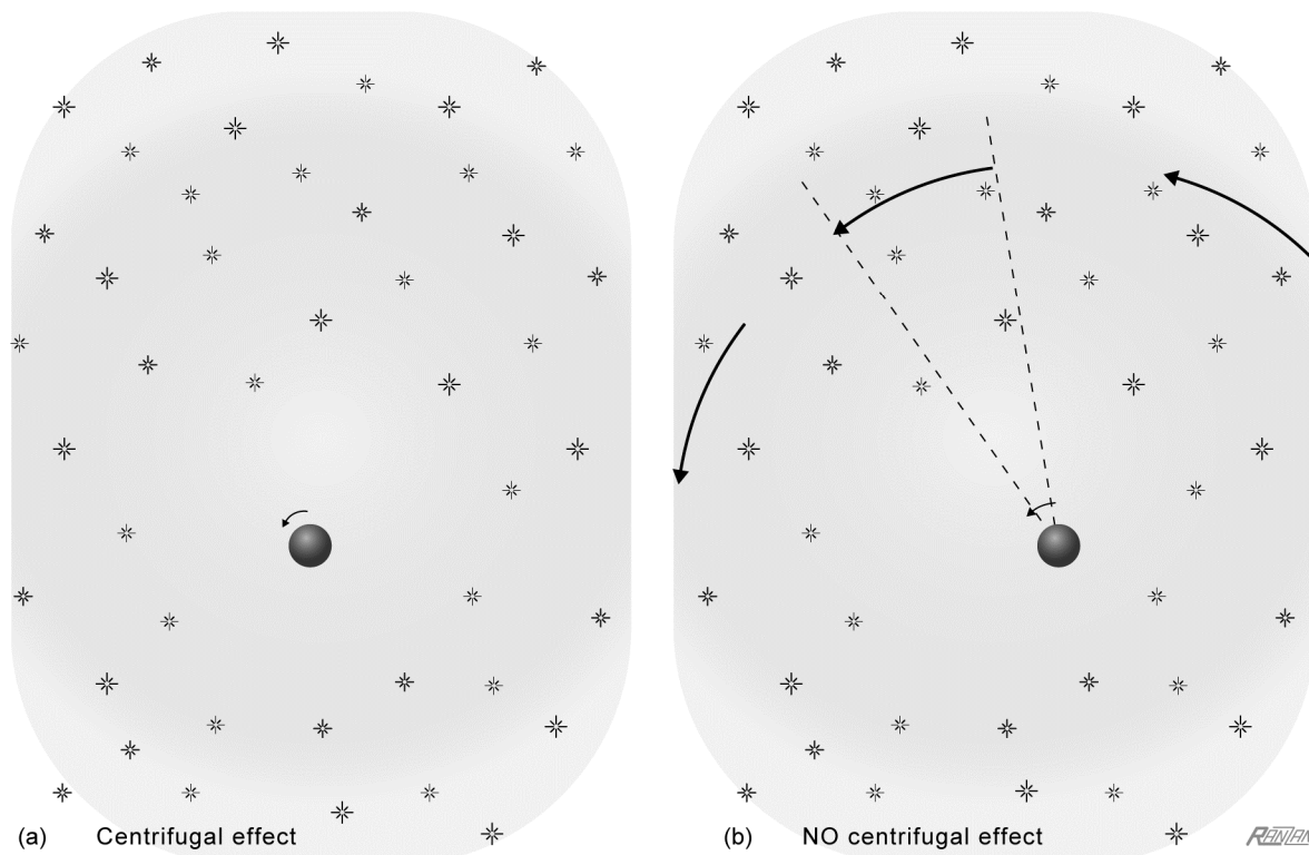
Figure 8. Mach’s hypothesis. (a) Body rotates relative to the background universe, “relative to the distant stars.” According to Ernst Mach, this is the cause of the inertial centrifugal effect. (b) Mach’s premise logically means that if the background universe were to rotate in synch with the test body, then there would be no centrifugal effect.
