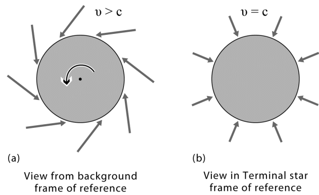
Figure 9. Rotating Terminal star from two perspectives. In (a), the view is with respect to background Euclidean space (space as an empty container) and shows significant aether dragging. The velocity magnitude of the flow must necessarily be greater than lightspeed. In (b), the view is in the frame of the spinning star; and regardless of the rotation rate, the flow speed at the surface is always the speed of light and the flow direction is always perpendicular to the surface. From the perspective of the Terminal star, the situation is equivalent to having the external world rotating in exact harmony WITH the star —essentially the star senses NO rotation whatsoever.
