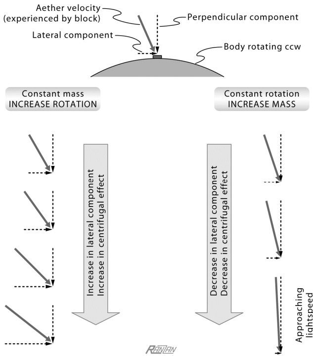
Figure 12. Key element in the cause of centrifugation is the presence of a lateral-motion component vector. Left column: With an increase in rotation, there is a corresponding increase in the lateral component; and, clearly, the centrifugal force must increase. Right column: However, with an increase in mass (of the gravitating body), there is a decrease in the lateral component; for logical consistency, the centrifugal effect must decrease. Note, the view (and the vector analysis) is within the frame of the rotating body. Rotation is counterclockwise.
