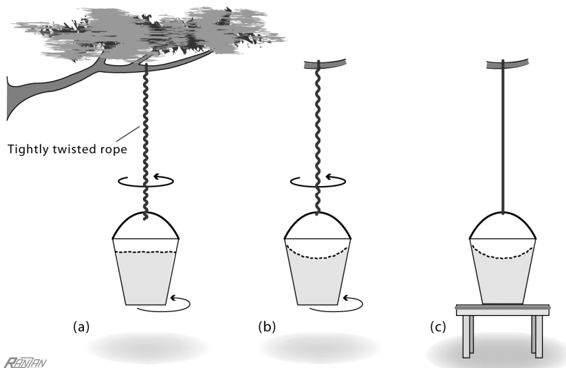
Figure 7. Newton's water-bucket experiment. Part (a) shows the situation just a brief moment after the bucket is released and allowed to spin in response to the torque present in the rope. At this stage, the water remains stationary while the bucket rotates around it; the water displays no centrifugal effects. In (b), the water displays a centrifugal effect (while rotating relative to the surrounding world), indicating the presence of absolute rotating motion. The surface of the water becomes concave, as it rises up the side of the bucket. In (c), the bucket is brought to a sudden stop. But the contents is still rotating, still manifesting the centrifugal effect of surface concaveness. Newton concluded that the centrifugal force is the result of absolute motion, not relative motion.
