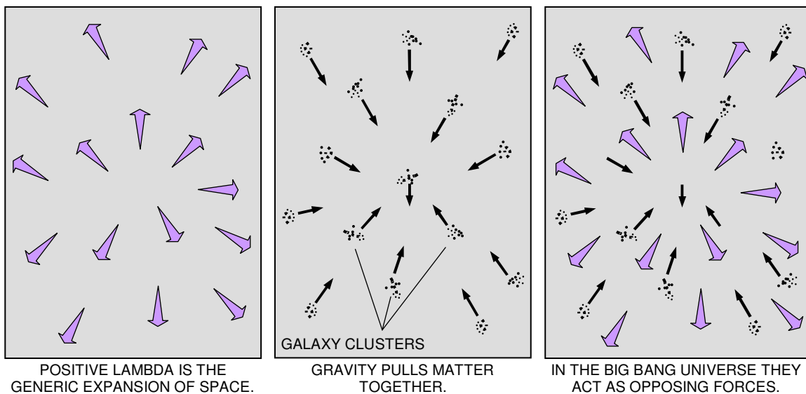
Fig. 1. Gravity and Lambda are treated as forces-in-opposition by the 20 th century cosmology. In the schematic representation of the BB universe, the two effects clearly behave as opposites in conflict.
