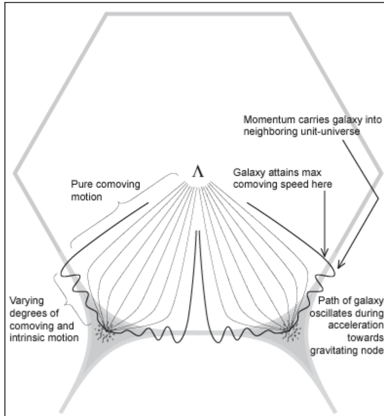
Fig. 7. Some trajectories deviate from pure comovement. In the Lambda region, galaxies (not shown) will accelerate towards the interface while gaining momentum. Since the motion of galaxies are subject to the law of inertia (Newton’s 1 st law of motion) those at, or near, the perimeter of the unified field will deviate considerably from comovement. A galaxy’s inertia —its reluctance to change its motion— propels it across the interface and into the neighboring cell. Gravity and \Lambda , however, are relentless; they dampen its wayward motion, guiding it towards the core of the node structure.
