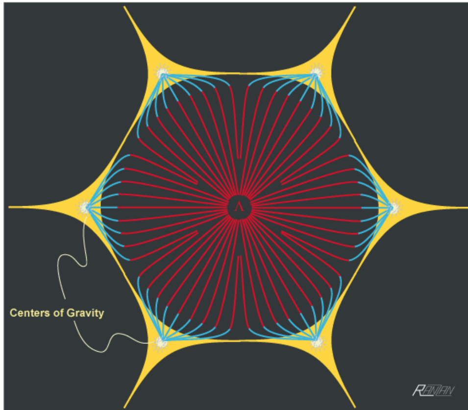
Fig. 5. Opposites in harmony in an idealized dynamic unit-universe (or cosmic cell). The curves are the trajectories of the movement of space itself and the idealized comovement of contained objects. There is a perpetual flow; first through the Lambda region (along the red paths); then through the gravitating region (along the blue paths) and into the very cores of the nodal galaxy clusters. (The hexagon is a schematic cross-section of a single cell of the DSSU.)
