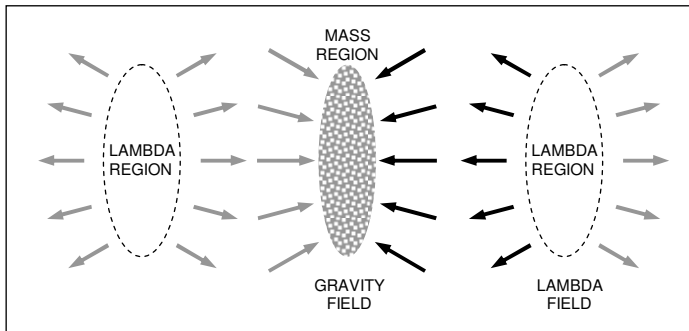
Fig. 3. Amplification of gravity and \Lambda posited for a non-expanding universe (i.e., \Lambda is not part of a Hubble flow). In the region between the centers of gravity and \Lambda , the two effects clearly reinforce each other. Force (field) vectors have components with a common direction.
