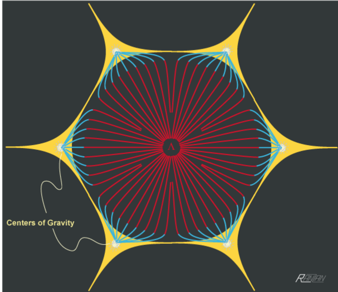
Fig. 5. Opposites in harmony in an idealized dynamic Unit-Universes. The curves are the trajectories of the movement of space itself and the idealized comovement of contained objects. There is a perpetual flow; first through the Lambda region (along the red paths); then through the gravitating region (along the blue paths) and into the very cores of the nodal galaxy clusters. (The hexagon is a schematic cross-section of a single cell of the DSSU.)
