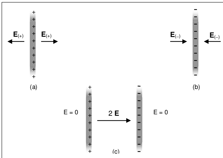
Fig. 2. Amplification of the electric field depends on the configuration. (a) and (b) Large nonconducting charged sheets viewed edge-on, and their associated electric fields. (c) The superposition of the two fields reveals a region where ‘opposites’ act in harmony.
