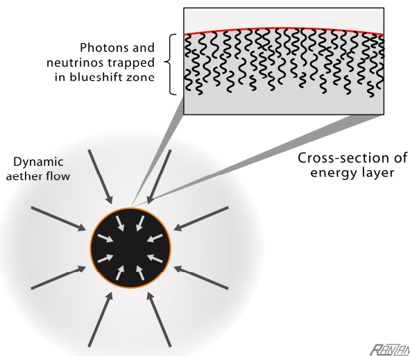
Fig. 5. The end-state neutron star has a unique surface layer. It is a thin zone consisting of photonic energy (gamma photons) and neutrinos. These particles are propagating outward; but because the aether is flowing inward with the same speed, the photons and neutrinos simply remain stationary within the energy layer. The crucial aspect is that the propagation is happening within a blueshifting region (in accordance with the Principle of velocity differential propagation). Consequently, the particles undergo energy amplification —they slowly gain energy.
