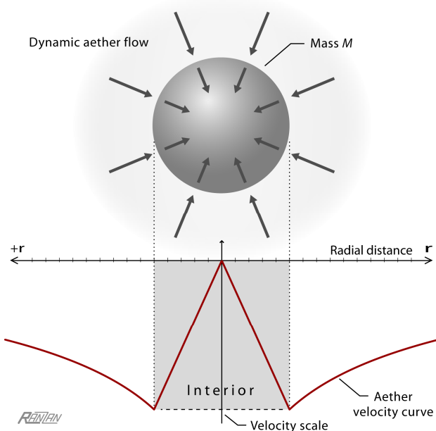
Fig. 1. Schematic of the gravity well (top) shows the flow of aether into the central mass. The body is not rotating, and is not moving with respect to the surrounding space medium. The aether flow profile (bottom) is linear for the interior of the structure; this is because the density is being treated as constant.
