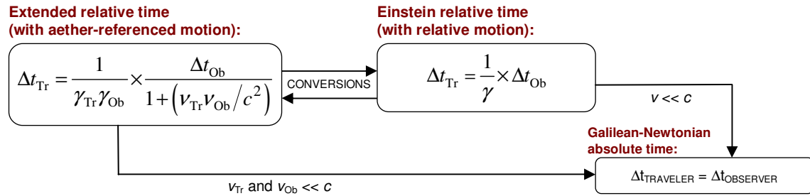
Fig. 9. Extended relativity time equation and how it relates to special relativity and classical relativity . When all speeds are restricted to low speeds the equations reduce to the classical Galilean-Newtonian form. (The “conversion” procedure is described in the text. The Lorentz factors are detailed in Table V.)
