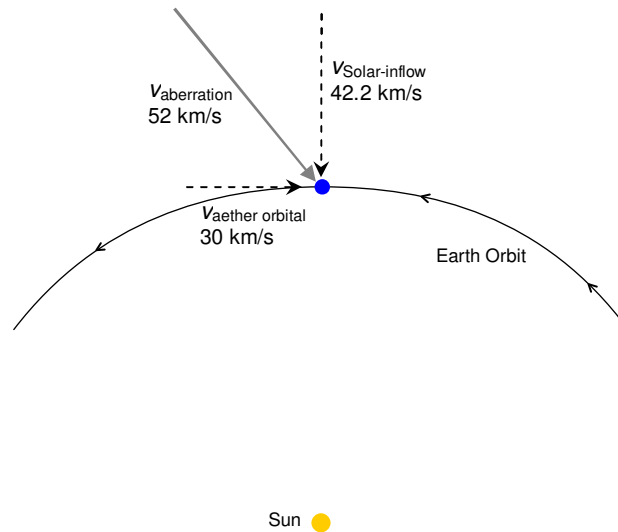
Fig. 7. Determining the net aether velocity (with respect to Earth) in the plane of the ecliptic. The motion component, v_{\text{aether orbital}} , and the gravitational component, v_{\text{Solar-inflow}} , when combined will serve as the net aberration velocity of 52 km/s. The Solar-inflow aether-vector is equal to the negative of the escape velocity, with respect to the Sun, at the distance of Earth's orbit.
