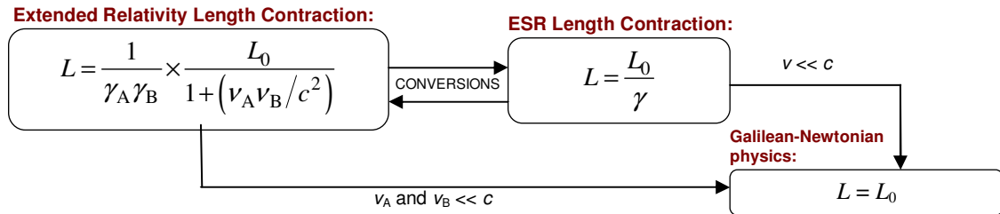
Fig. 10. Extended relativity length-contraction equation and how it relates to special relativity and classical physics. When speeds are restricted to low speeds the equations reduce to the Galilean-Newtonian form. (The “conversion” procedure is described in the text. The Lorentz factors are detailed in Table V.)
