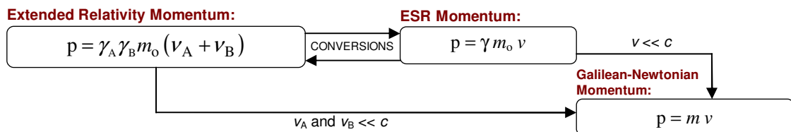
Fig. 11. Extended relativity momentum equation and how it relates to special relativity and classical physics. When speeds are restricted to low speeds the equations reduce to the Galilean-Newtonian form. (The “conversion” procedure is described in the text. The Lorentz factors are detailed in Table V.)
