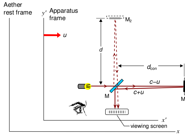
Fig. 3. Analysis of the speed of light waves along the “parallel” arm of a vac-mode Michelson interferometer (schematic plan view). The arm is parallel to the direction of absolute motion (i.e., motion through aether-space) and therefore undergoes actual length contraction. The contracted length is labeled as d_{\text{con}} .
