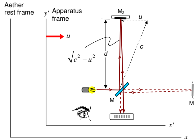
Fig. 4. Analysis of the velocity of light waves along the “perpendicular” arm of a vac-mode Michelson interferometer (schematic plan view). According to the aether-space theory, the light wave going from M to M_2 travels with speed c with respect to aether along the diagonal dashed path. But it travels with speed (c^2 - u^2)^{1/2} with respect to the “moving” Apparatus/observer frame —as shown by the velocity-vector triangle. A similar analysis applies to the wave going from M_2 back to M .
