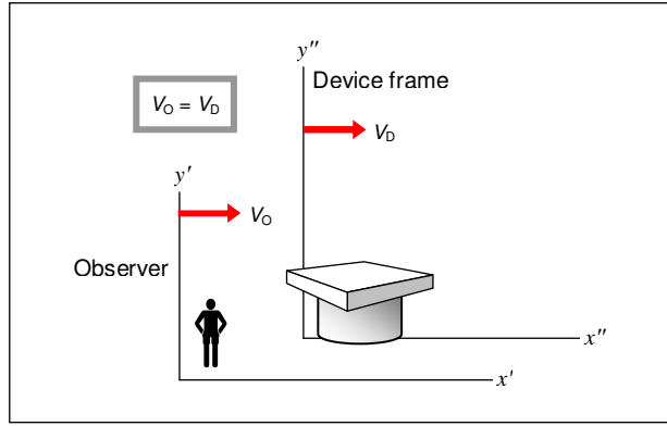
Fig. 2. No length contraction observed under tandem motion. The Observer has absolute motion towards the other frame; therefore, according to the sign rule, v_O is ‘-’. The interferometer device has absolute motion away from the other frame; thus v_D is ‘+’. The length contraction eqn (1) then reduces to L_{\text{apparent}} = L_0 .
